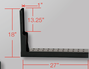
TBP010 Single L-arm center support for 78" toolboxes or mounting dual boxes 27" x 18"
