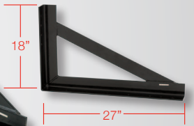
TBP008 One pair of Heavy Duty L-arm mounting brackets 27" x 18"
