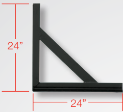
TBP002 One pair of Heavy Duty L-arm mounting brackets 24" x 24"
