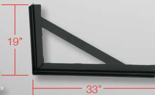
TBP006 Single Heavy Duty toolbox sandwich bracket with mounting hardware 33" x 19"
